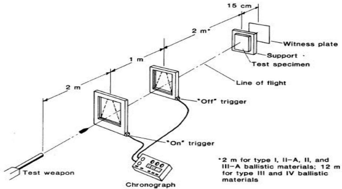
FIGURE 2. Ballistic test setup
